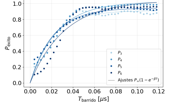
(b) P_n , A = 100 \text{ rad}/\mu\text{s}
