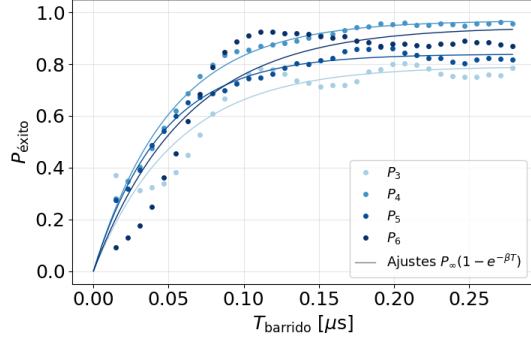
(a) P_n , A = 50 \text{ rad}/\mu\text{s}
